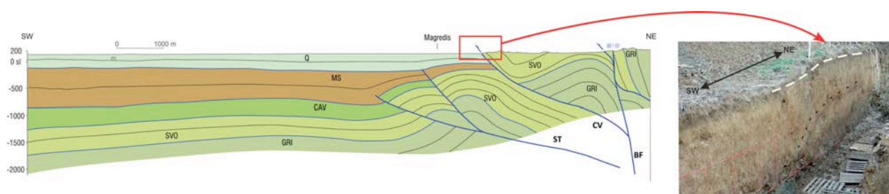
Figure 1. Geological cross-section crossing the Borgo Faris and Colle Villano faults, left panel; Legend: Q: Plio(?)–Quaternary succession; MS: Upper Miocene Molassa; CAV: Lower Miocene Molassa; SVO: Savorgnano marls and sandstones (Ypresian p.p.); GRI: Grivò Flysch (Thanetian? – Ypresian p.p.). ST: Susans-Tricesimo thrust; CV: Colle Villano thrust; BF: Borgo Faris strike slip fault. Northern wall of one of the trenches dug across the Colle Villano fault; white dashed line marks the scarp at surface; black dashed line marks the bending affecting the sedimentary sequence exposed by the trench.
